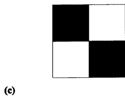
Figure 4. Molecular structure of 10a ( RSSR ); (a) front-view: square-planar environment of Pd II ; (b) side-view: C 2 -symmetric arrangement; hydrogen atoms have been omitted for clarity; (c) quadrant diagram
