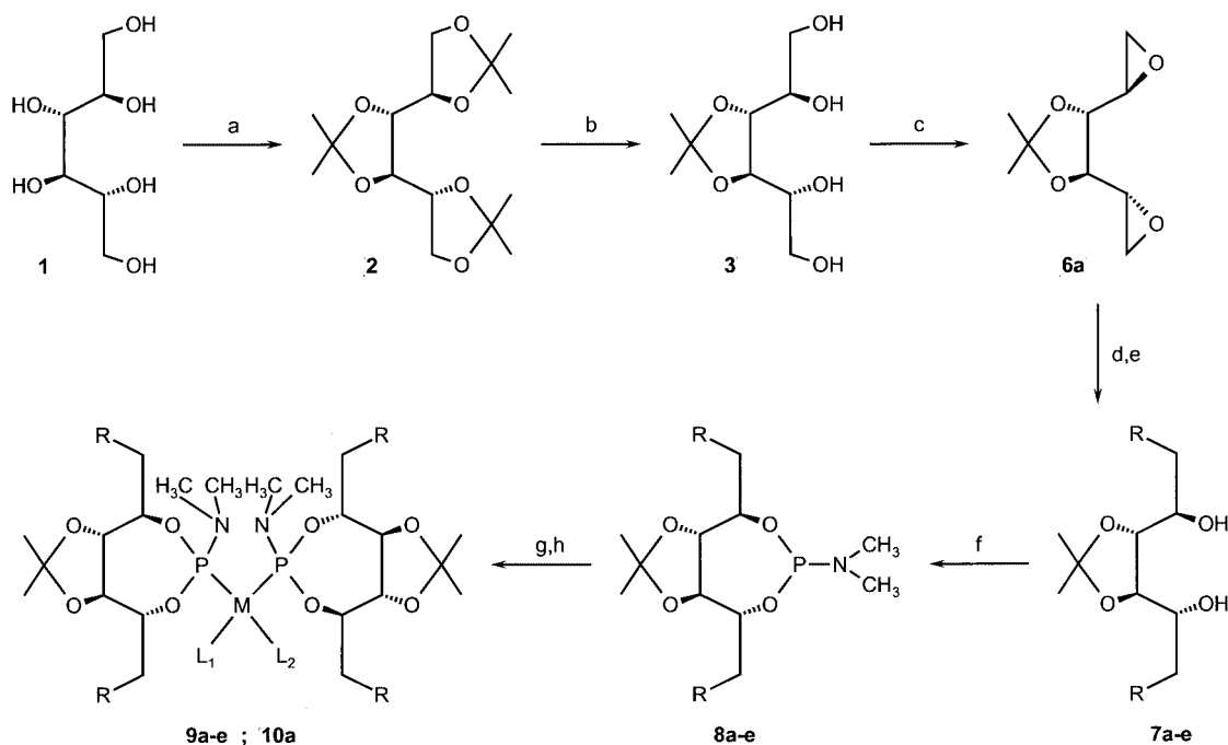
Figure 1. a) acetone, H 2 SO 4 ; b) AcOH, H 2 O, 40 °C; c) (i) trimethyl orthoacetate, PPTS, (ii) NEt 3 , AcBr, (iii) K 2 CO 3 , MeOH; d) LiAlH 4 , Et 2 O, R = H (7a); e) CuBr·SMe 2 , RMgBr, THF/Et 2 O, -40 °C, R = CH 3 (7b), C 2 H 5 (7c), i C 4 H 9 (7d), C 6 H 5 (7e); f) HMTAP, toluene, reflux; g) [Rh(COD) 2 ][SO 3 CF 3 ], CH 2 Cl 2 , 9a-e: M = Rh, L 1 -L 2 = COD; h) [PdCl 2 (COD)], CH 2 Cl 2 , 10a: M = Pd, L 1 = L 2 = Cl
