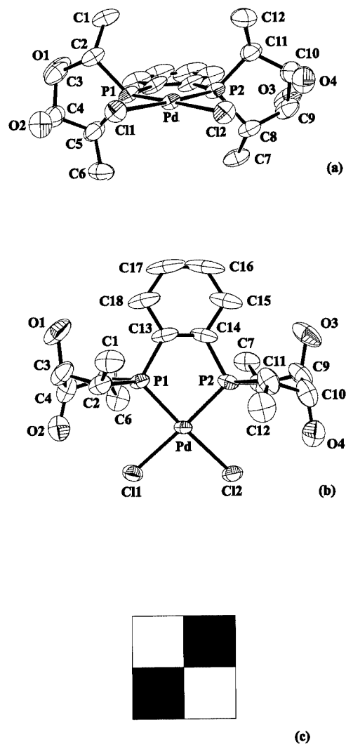
Figure 6. Molecular structure of 15a ( SSSS ); (a) front-view: square-planar environment of \text{Pd}^{\text{II}} ; (b) top-view: C_2 -symmetric arrangement; hydrogen atoms have been omitted for clarity; (c) quadrant diagram
