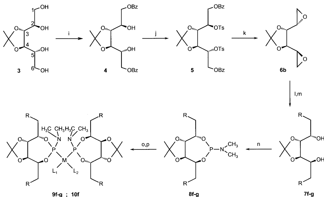
Figure 2. i) benzoyl chloride, pyridine, CH 2 Cl 2 , -80 °C; j) tosyl chloride, NEt 3 , 4-(dimethylamino)pyridine, CH 2 Cl 2 ; k) K 2 CO 3 , MeOH; l) LiAlH 4 , Et 2 O, R = H (7f); m) CuBr·SMe 2 , PhMgBr, THF/Et 2 O, -40 °C, R = C 6 H 5 (7g); n) HMTAP, toluene, reflux; o) [Rh(COD) 2 ][SO 3 CF 3 ], CH 2 Cl 2 , 9f-g: M = Rh, L 1 -L 2 = COD; p) [PdCl 2 (COD)], CH 2 Cl 2 , 10f: M = Pd, L 1 = L 2 = Cl
