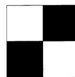
Figure 5. Molecular structure of 10f ( SSSS ); (a) front-view: square-planar environment of Pd II ; (b) side-view: C 2 -symmetric arrangement; hydrogen atoms have been omitted for clarity; (c) quadrant diagram
